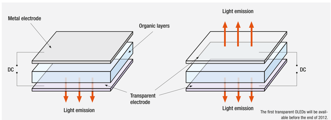
Two different OLED designs: emission from one side on the left, and emission from both sides on the right.
